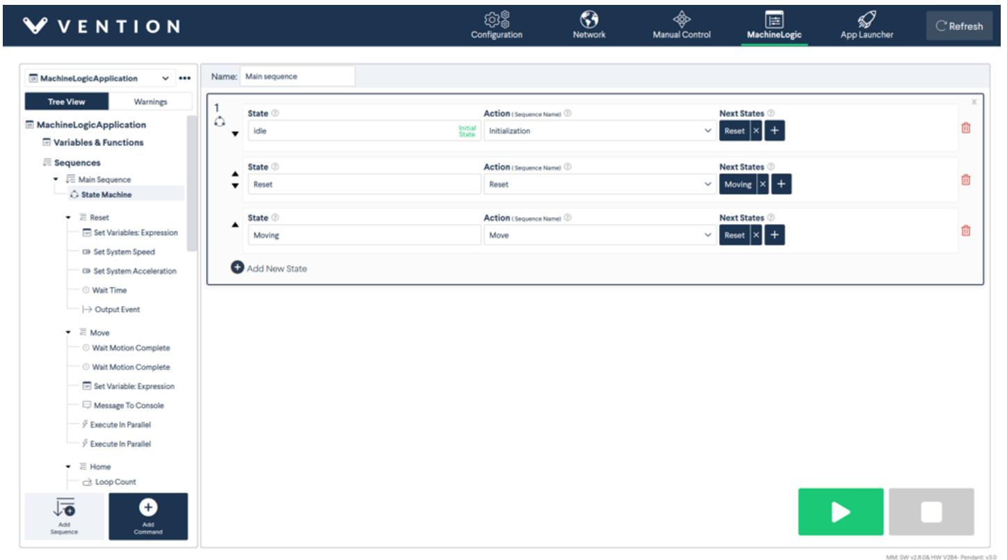
Figure 3: MachineLogic
