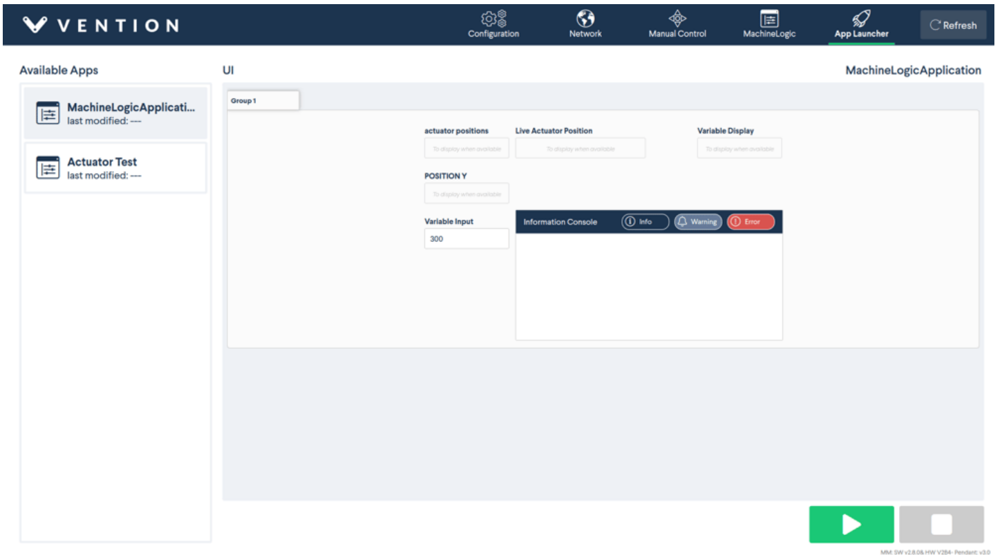
Figure 4: Application Launcher
