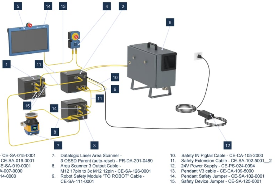
Figure 5 - Auto-reset with no MachineMotion wiring diagram
