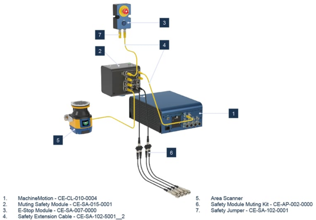
Figure 9 - Muting kit wiring diagram
