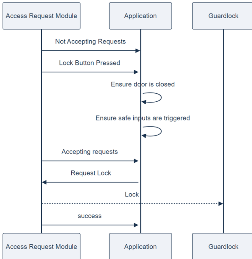
Figure 3: Successful lock sequence
