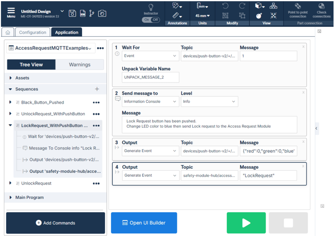
Figure 13: MachineLogic example to handle a button being pushed to trigger the lock request and send that command to the Access Request Module
