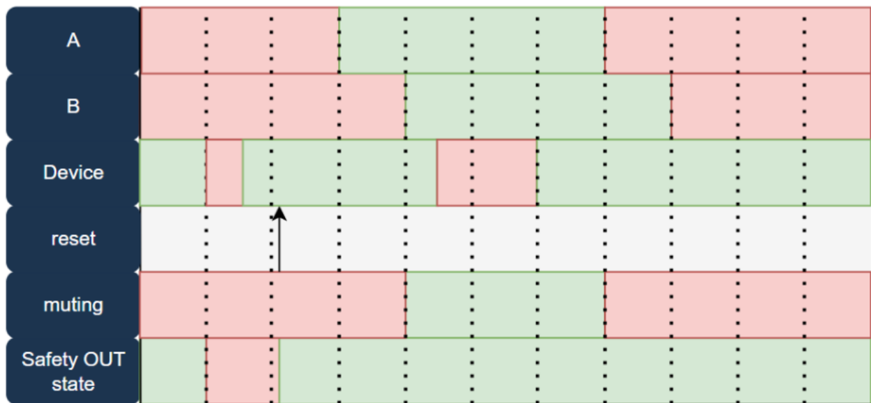
Figure 2: Muting Logic
