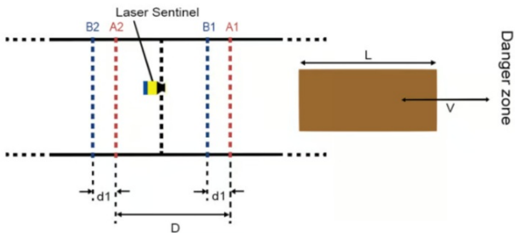
Figure 3: Bi-directional muting
