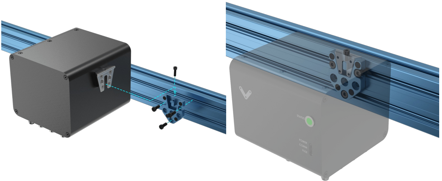
Figure 5: Module Mounting
